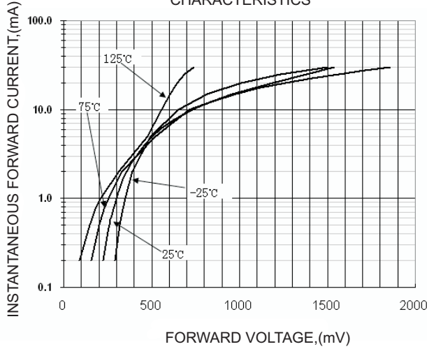
FIG.1-TYPICAL FORWARD CHARACTERISTICS
